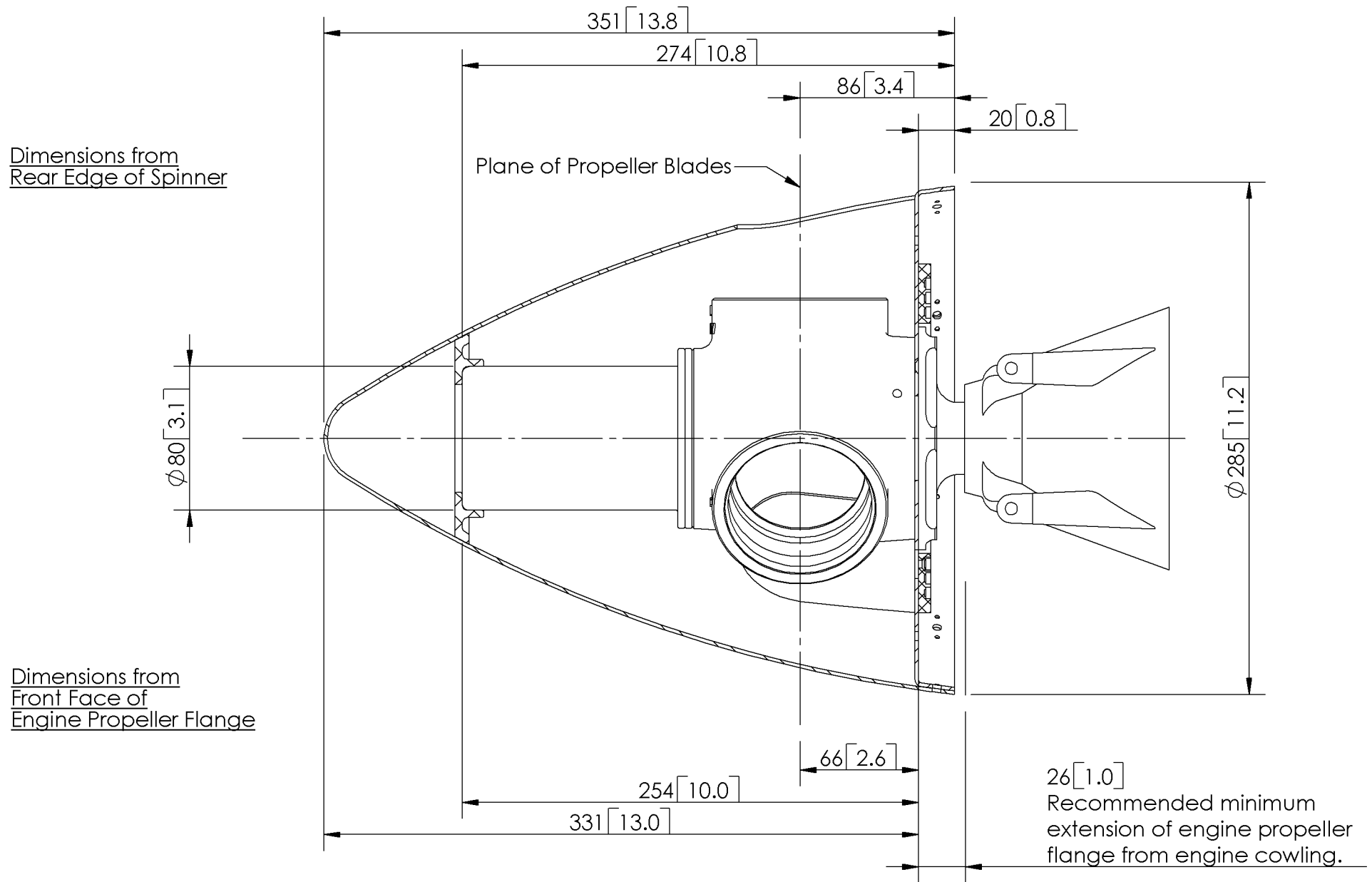
Principal Dimensions of AP332 Propeller with \phi 285\text{mm} (11.2in) Spinner (Example shown mounted on Rotax engine) Primary dimensions in millimeters [secondary dimensions in inches]
